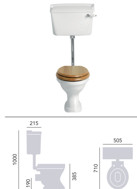
Low Level WC and Cistern
