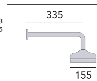
Large 6" shower head.
