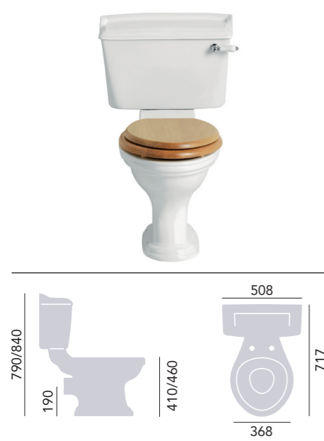
Close Coupled WC & Landscape Cistern
