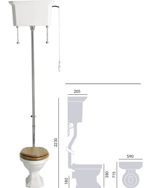
High Level WC and Cistern
